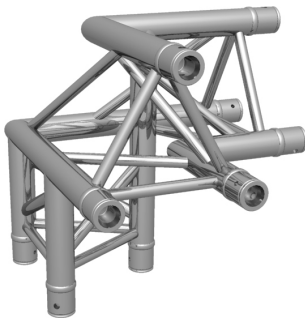
F33 3-Wege Ecke 90° oben/links F33 3-way corner 90° top/left
