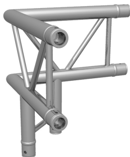
F32 3-Wege 90° vertikal F32 3-way 90° vertical
