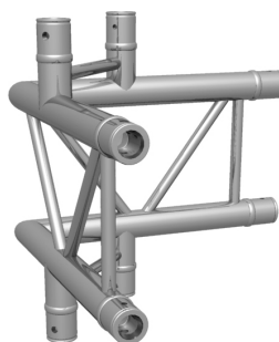
F32 4-Wege Ecke vertikal F32 4-way corner vertical
