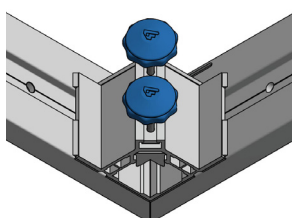
Leg Attachment Corner (welded)
